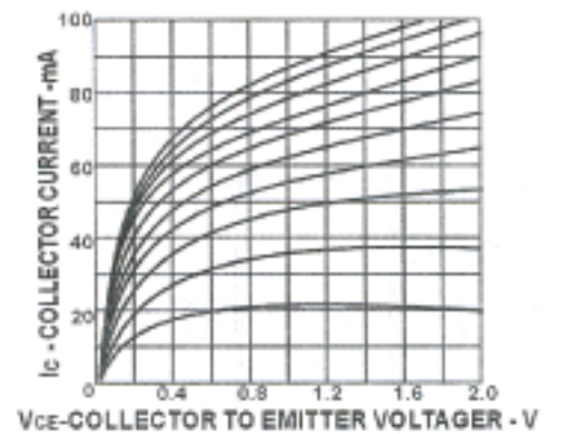
FIG2. Collector Current vs Collector to Emitter Voltage
